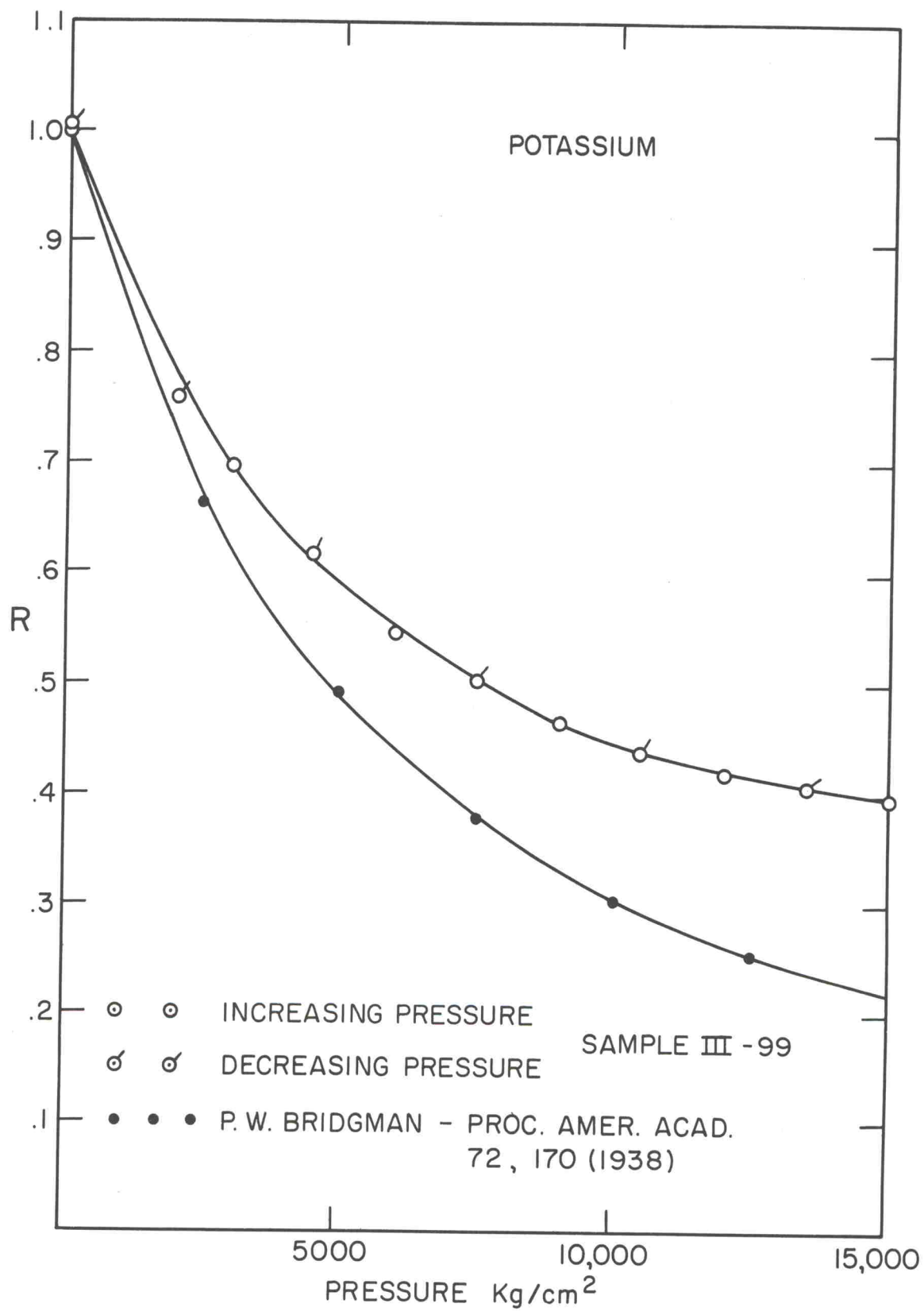
FIG. 3-6 NORMALIZED RESISTANCE R, vs. PRESSURE
